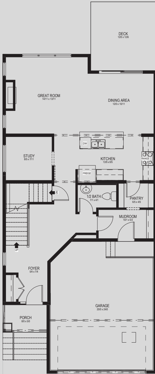
Main Floor - 1023 sqft
