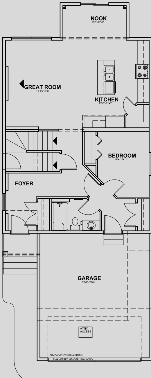
Main Floor - 956 sqft
